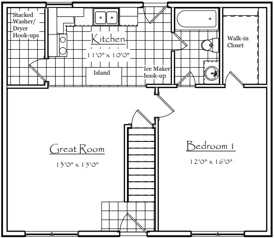
1 Bedroom First Floor
