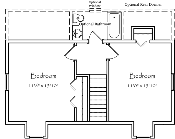
Optional Second Floor
