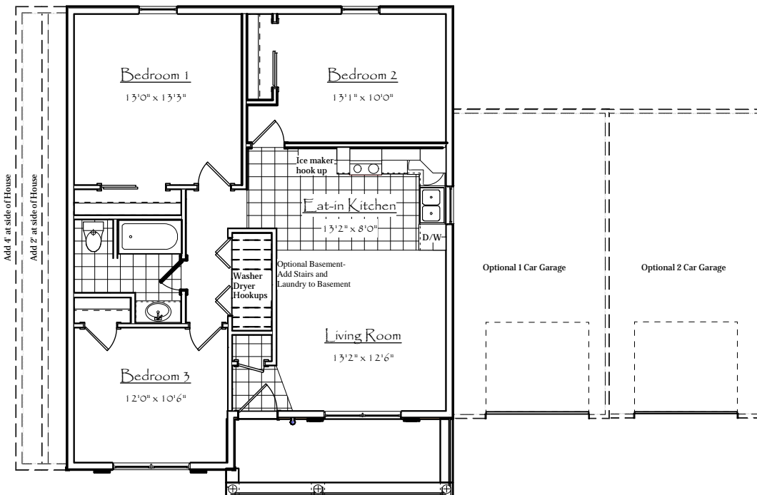
OPTION 2 FLOOR PLAN
