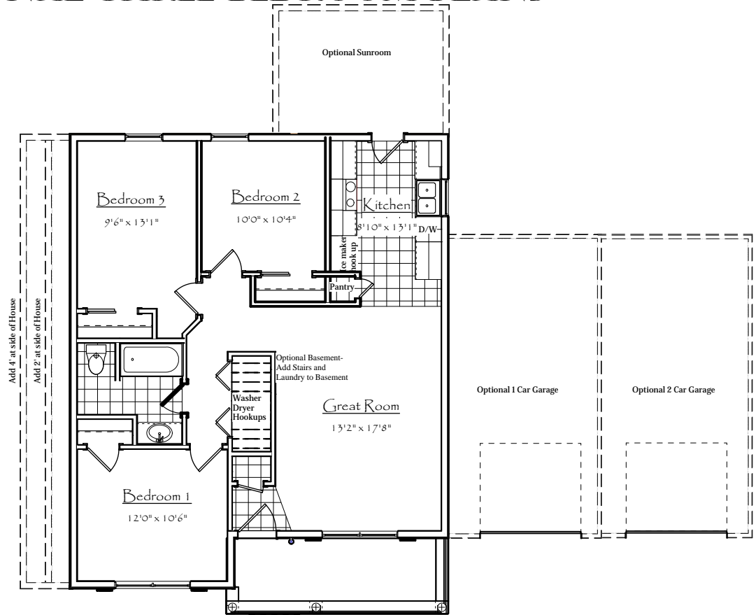
OPTION 1 FLOOR PLAN
