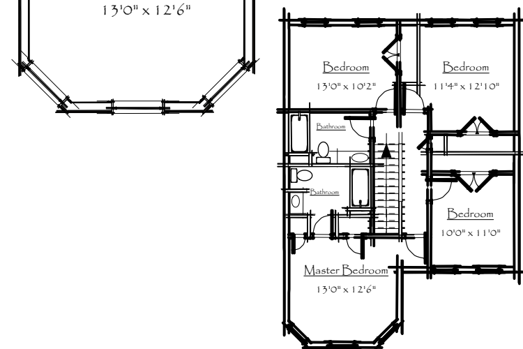
Optional 4 Bedroom Second Floor Plan
